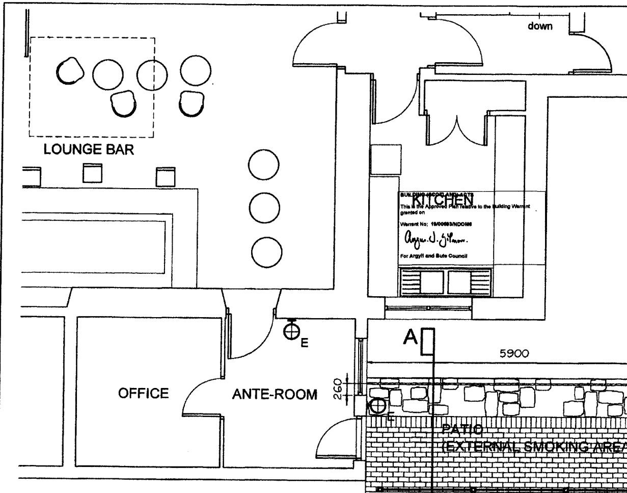
Floor Plan (part) Scale - 1:30
